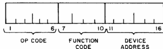
Figure 1-5. Input/Output Instruction Format
